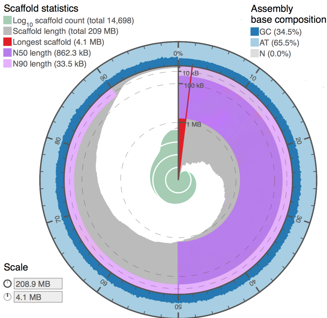
Figure 4 Genome assembly statistics visualization of Proctacanthus coquilleti de novo genome (w2rap-contiggen 200 kmer assembly, see also Table 5). Visualized at: http://lepbase.org/assembly-statistics/ , figshare doi: 10.6084/m9.figshare.4056042 .
